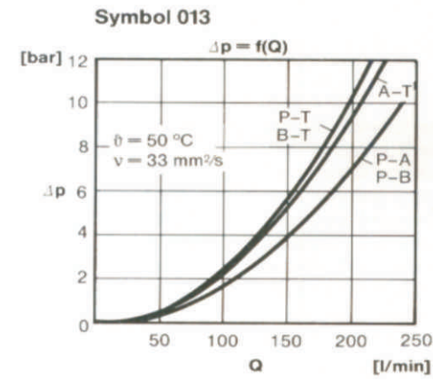
NG16 Curves
