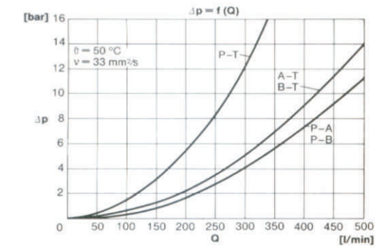
NG25 Curves
